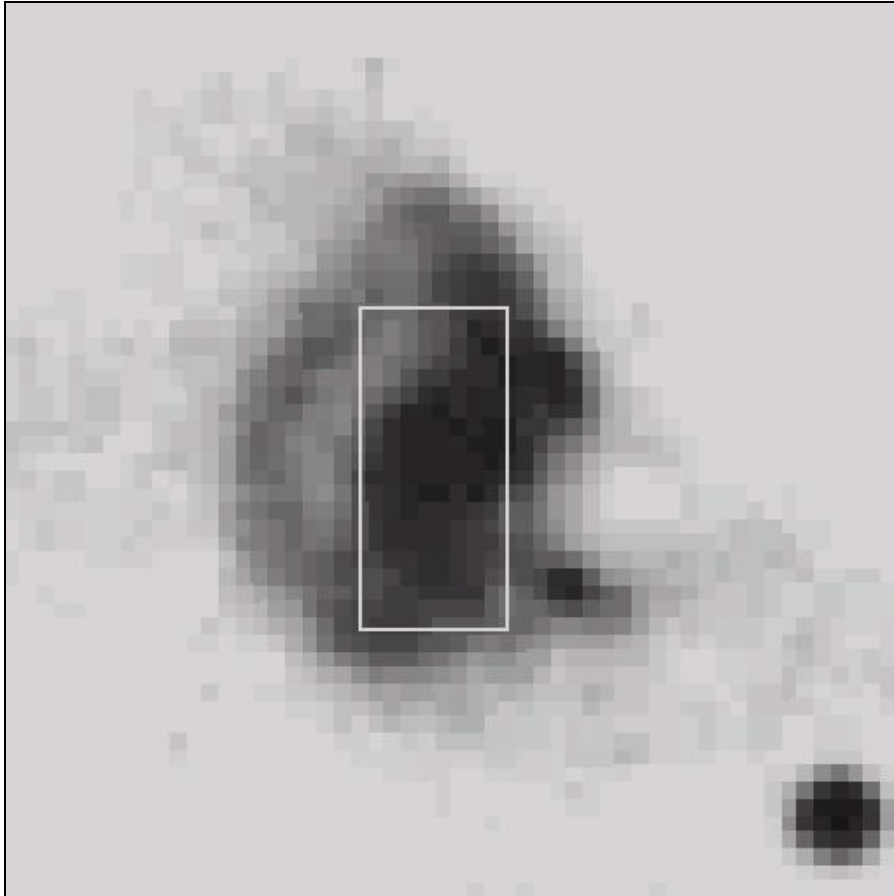
Figure 7 – POSS image of Markarian 538 overlaid with the FISICA IFU field-of-view. In a single shot, FISICA will provide R\sim 1300 1.5\text{-}2.4\ \mu\text{m} spectra of the entire central region of this luminous blue compact galaxy. Luminous Compact Blue Galaxies are starburst galaxies that have been recently identified as the local counterparts of the Lyman-break galaxy population at high redshifts. The spectral lines we wish to study include: [Fe II] (1.644 \mu\text{m} ), H 2 (2.122 \mu\text{m} ), and Br gamma (2.166 \mu\text{m} ). These new data will yield constraints on various characteristics of the star-forming episodes in these regions, including their strength, maturity, spatial variability, and extinction.
