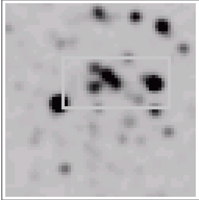
Figure 8 – 2MASS Ks-band image of the high-mass star cluster Cl1806-20, overlaid with the FISICA field-of-view. The FISICA region includes >10 high-mass stellar candidates which are too closely-spaced for efficient MOS spectroscopy. FISICA can provide spectroscopy of important lines ( Br\gamma , HeI, HeII, FeII, etc.) to identify the nature of these stars, as well as the extinction towards them, accomplishing in ~1-hour what would take ~1 night of observations with a conventional long-slit spectrograph.
