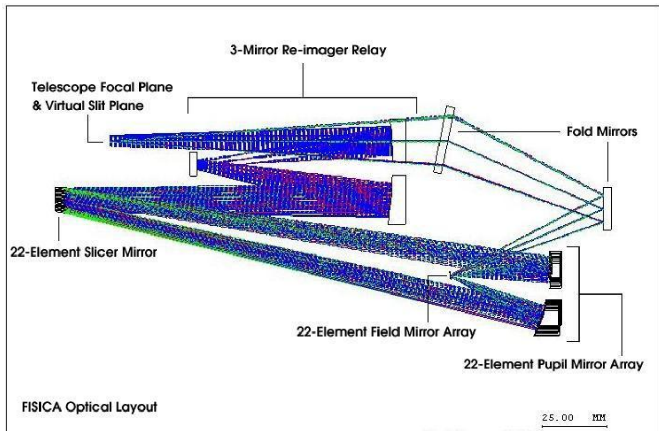
Figure 1 – Optical concept layout for FISICA
