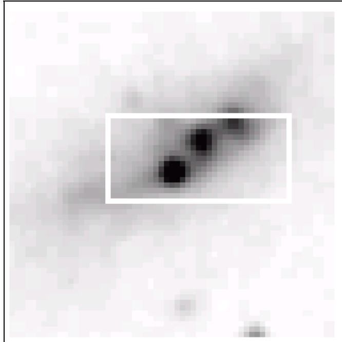
Figure 10 – 2MASS Ks-band image of nearby dwarf starburst galaxy NGC 1569. Note that a single pointing can obtain 1.5-2.4 \mu\text{m} spectra of the two major extended star clusters near the center of this galaxy.
