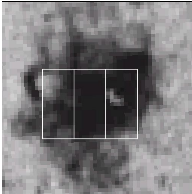
Figure 9 – POSS image of the super OB association NGC 604 in M33, overlaid with 3 contiguous FISICS fields-of-view. In just 3 separate exposures, FISICA can obtain 1.5-2.4 \mu\text{m} spectra of the entire core of this complex region, allowing identification of various stellar populations, ages, and extinction.
